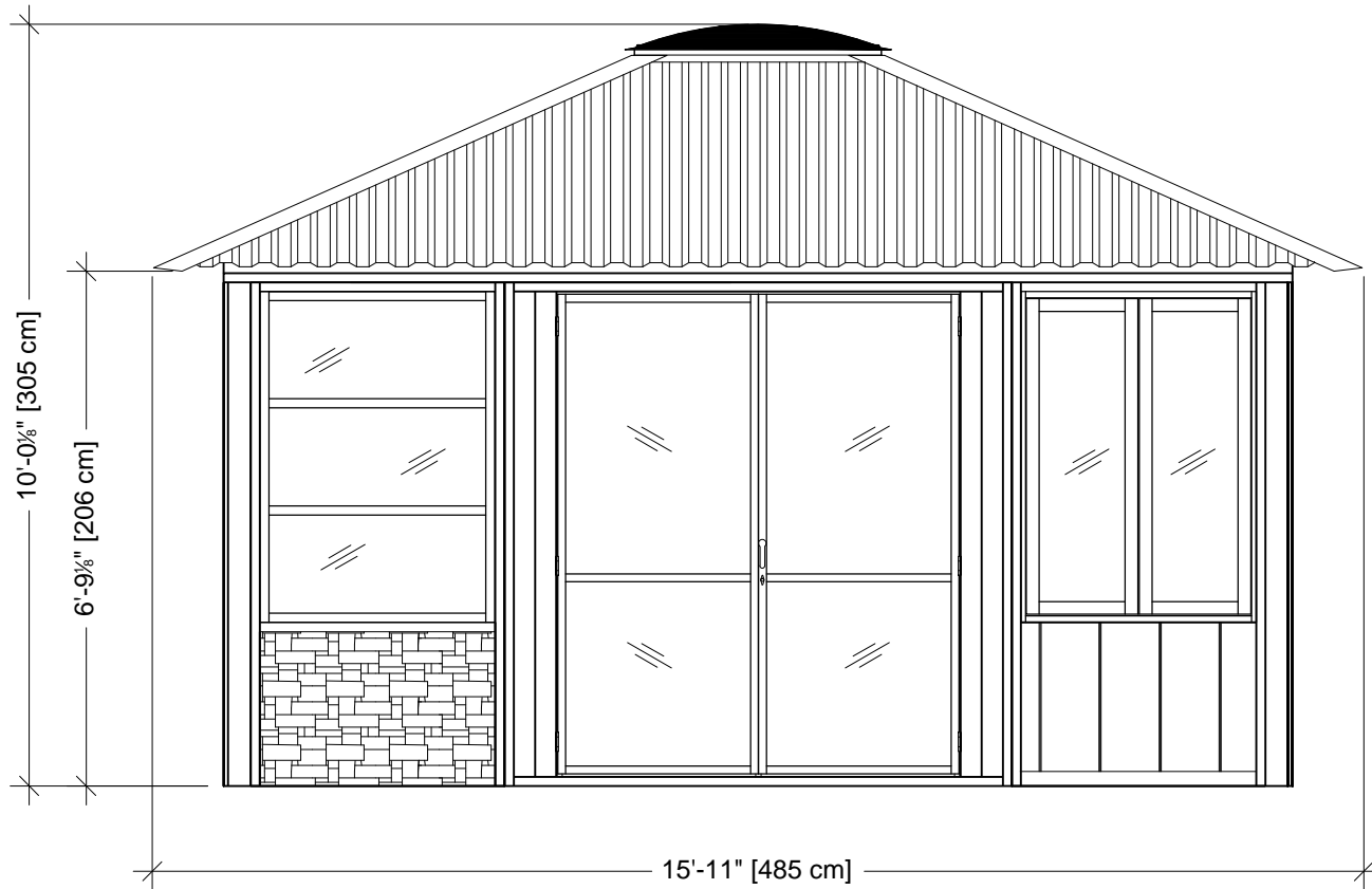
Front Elevation
