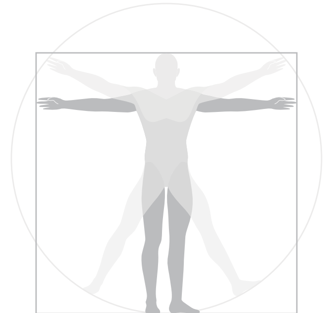
ANTHROPOMETRIC DIMENSIONS
